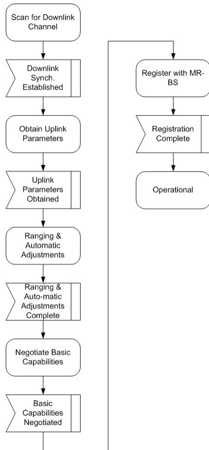
Figure 2. RS network entry procedure.
