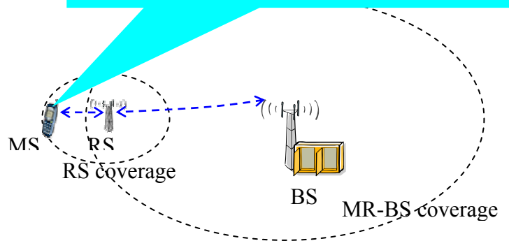
Fig.2 Non-Transparent RS
