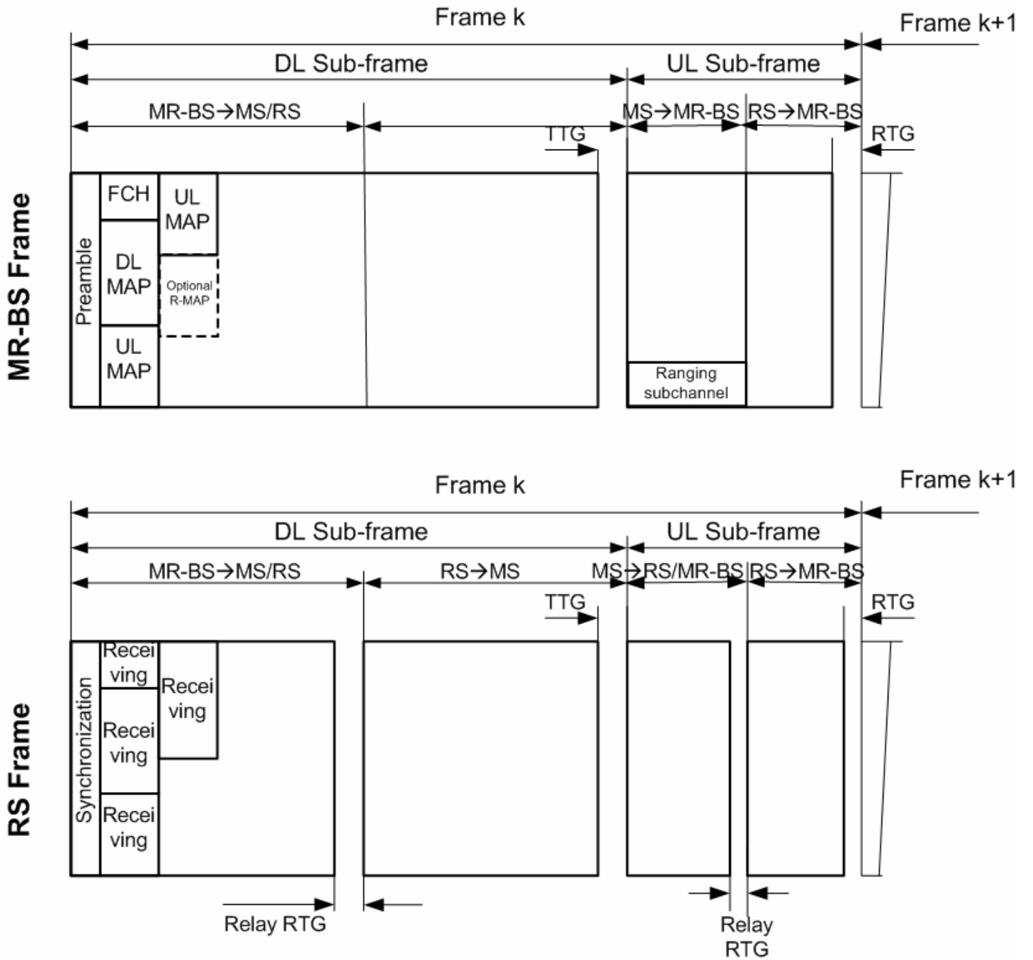
Figure xxx Example of minimum configuration for an in-band transparent relay frame structure
