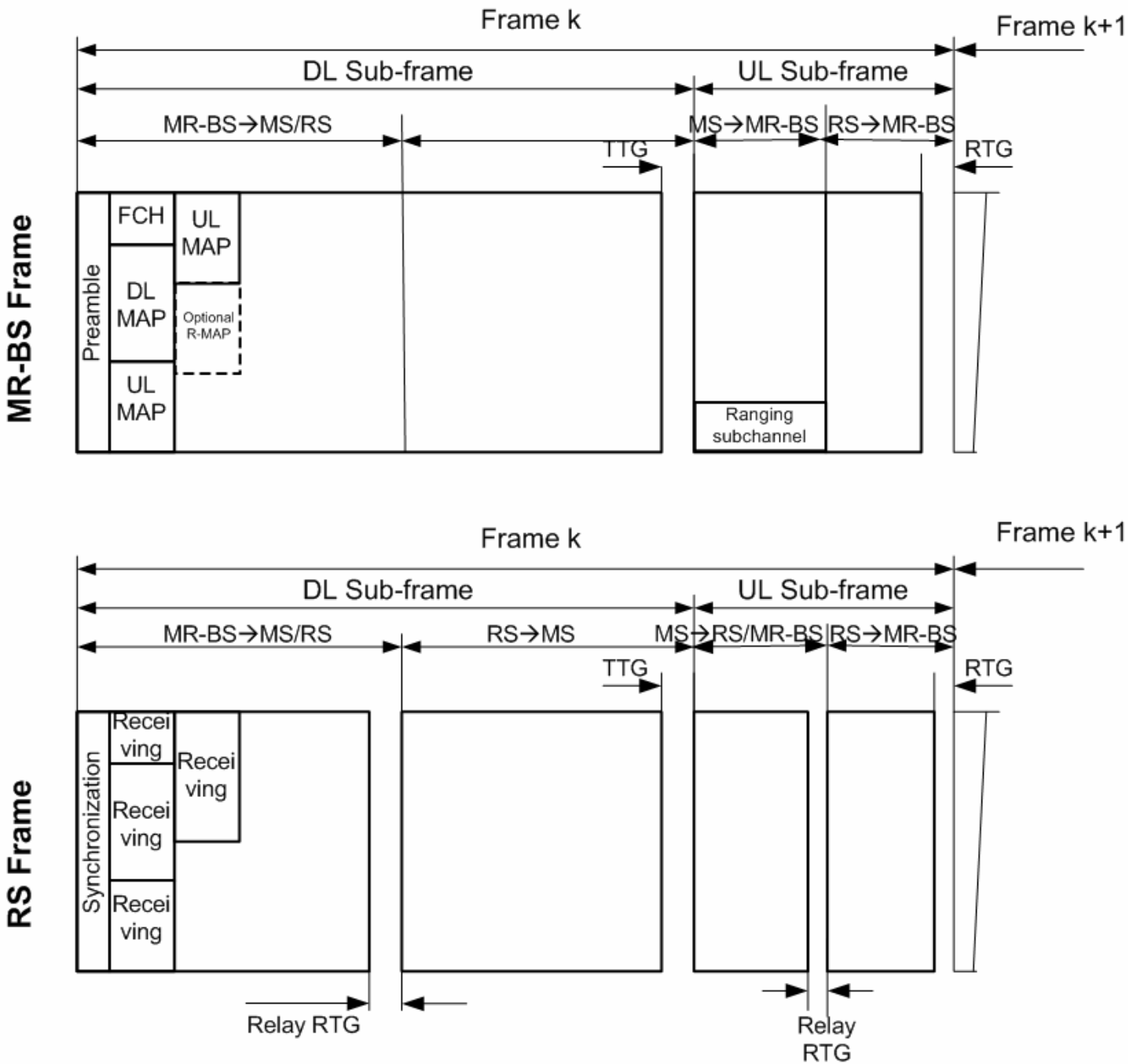
Figure.3. Example of minimum configuration for an in-band transparent relay frame structure
