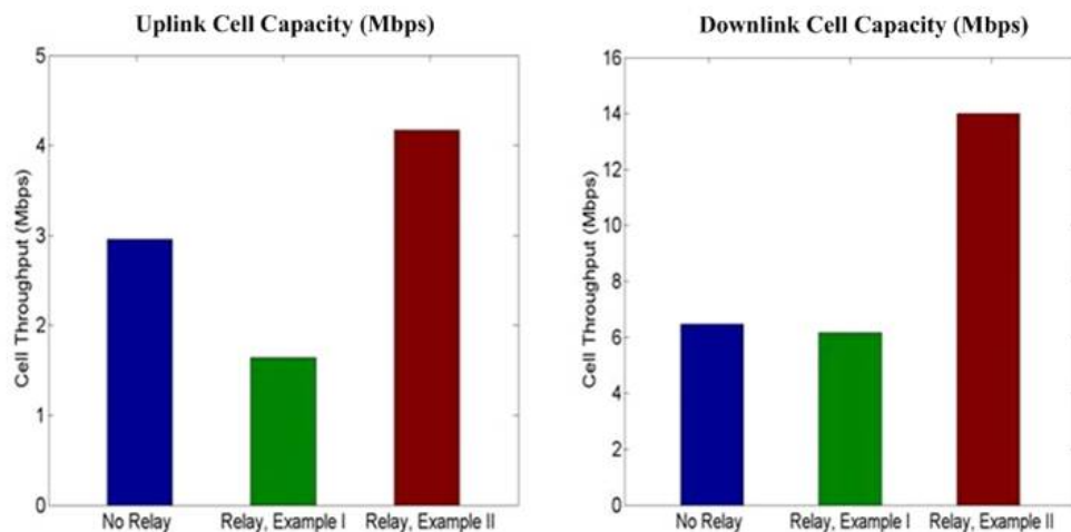
23 24 Fig.1 Capacity comparison for different relay scenarios
