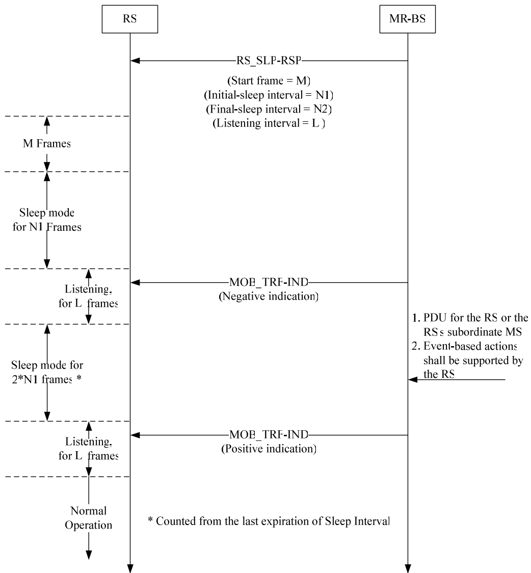
Figure D. 11--Example RS sleep mode — MR-BS initiated
