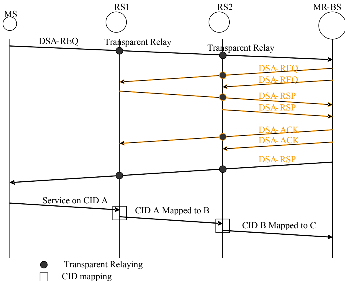
Fig.2. MR-BS initiated CSP setup triggered by MS initiated DSA-REQ with transparent forwarding
