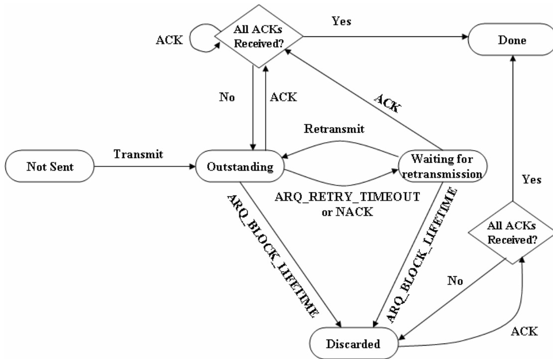
Figure 4 RMM-ARQ transmit block states
