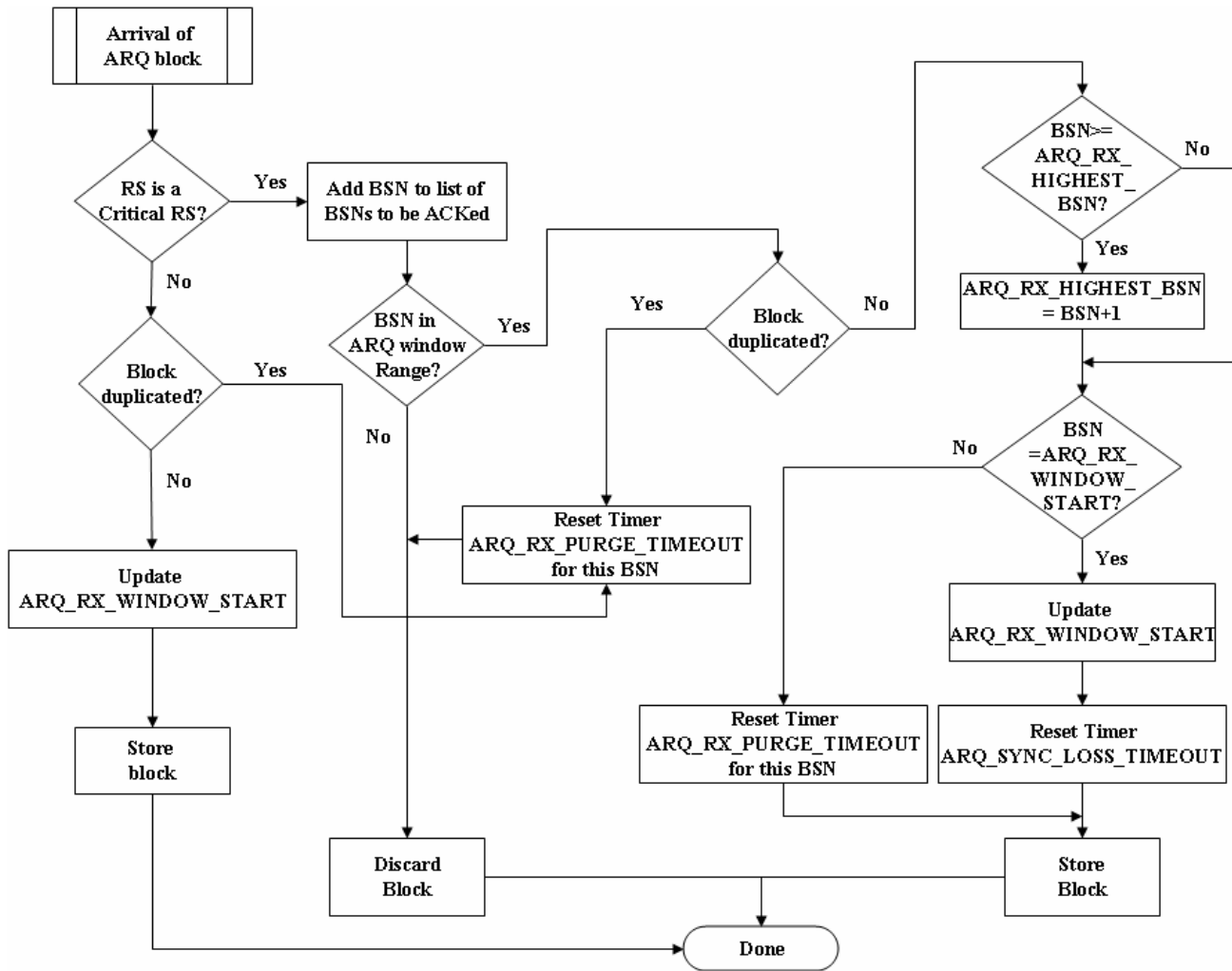
Figure 5 RMM-ARQ block reception
