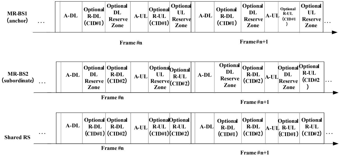
Fig.2 shared RS system for MMR.
