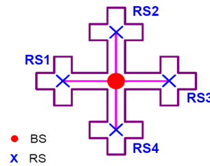
Fig.2 Manhattan Model
