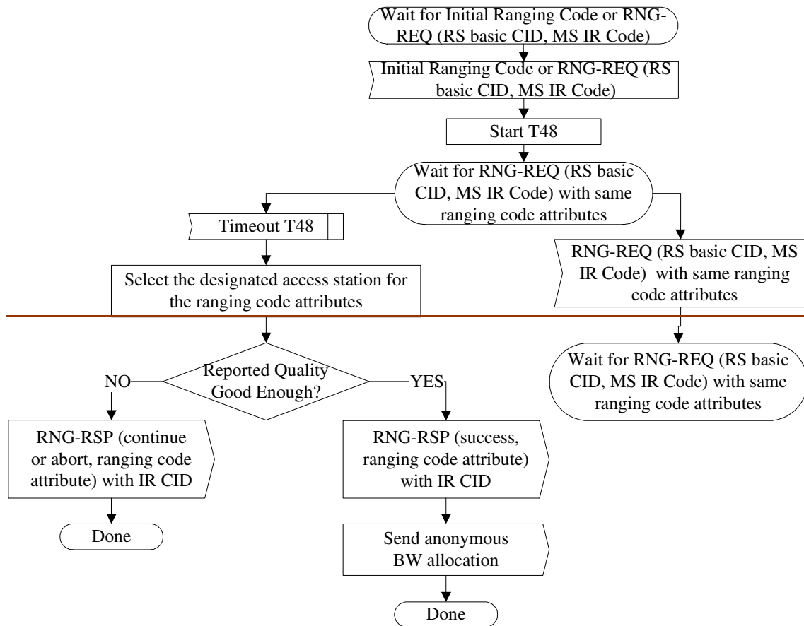
Figure 95c—MS CDMA Initial Ranging with Transparent RS—MR-BS
