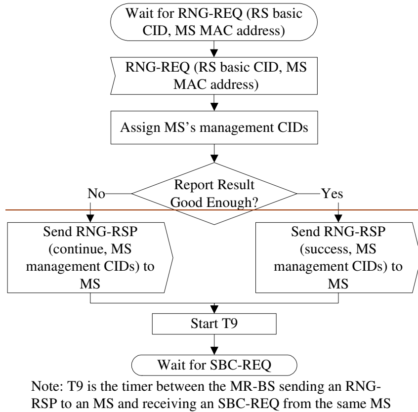
Figure 95d—MS Initial Ranging with Transparent RS—MR-BS
