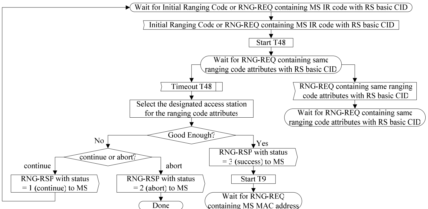
Figure 95c—Handle CDMA initial ranging code in transparent mode at MR-BS
