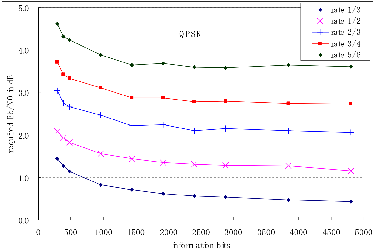
Performance for RC LDPC codes based on the 16e LDPC codes
