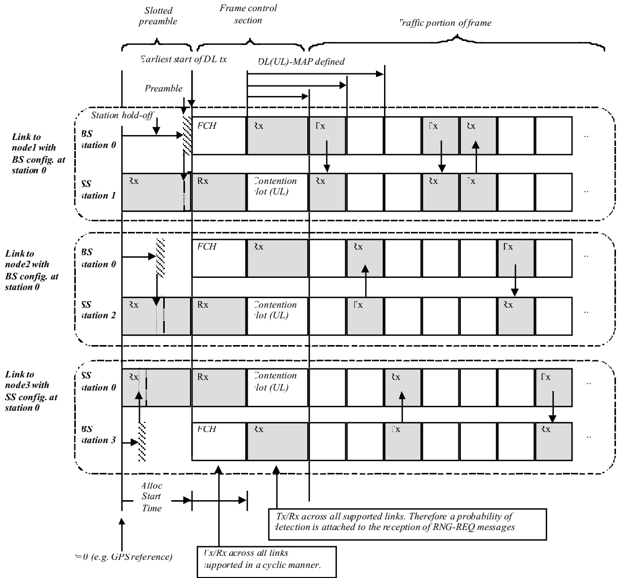
Figure 44 Configuration of links supported by station 0 and the multiple half links for H-FDD-like operation in IEEE802.16. NB Burst preambles are not shown, neither are TRGs. The diagram is not to scale.
