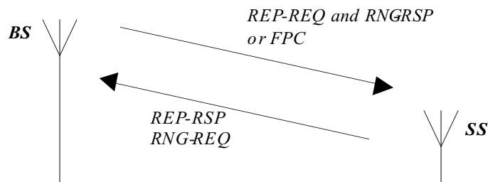
Figure 55 Configuration of MAC messages used in power control.
