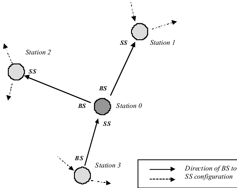
Figure 33 Example configuration for station 0. NB all links shown are duplex links, the arrowheads show BS to SS link termination orientation.
