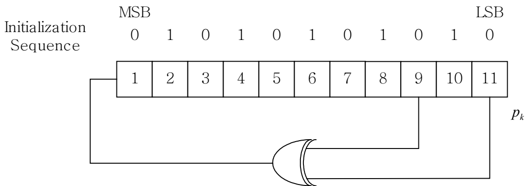
Figure 3: PRBS structure for preamble and pilot symbol generation
