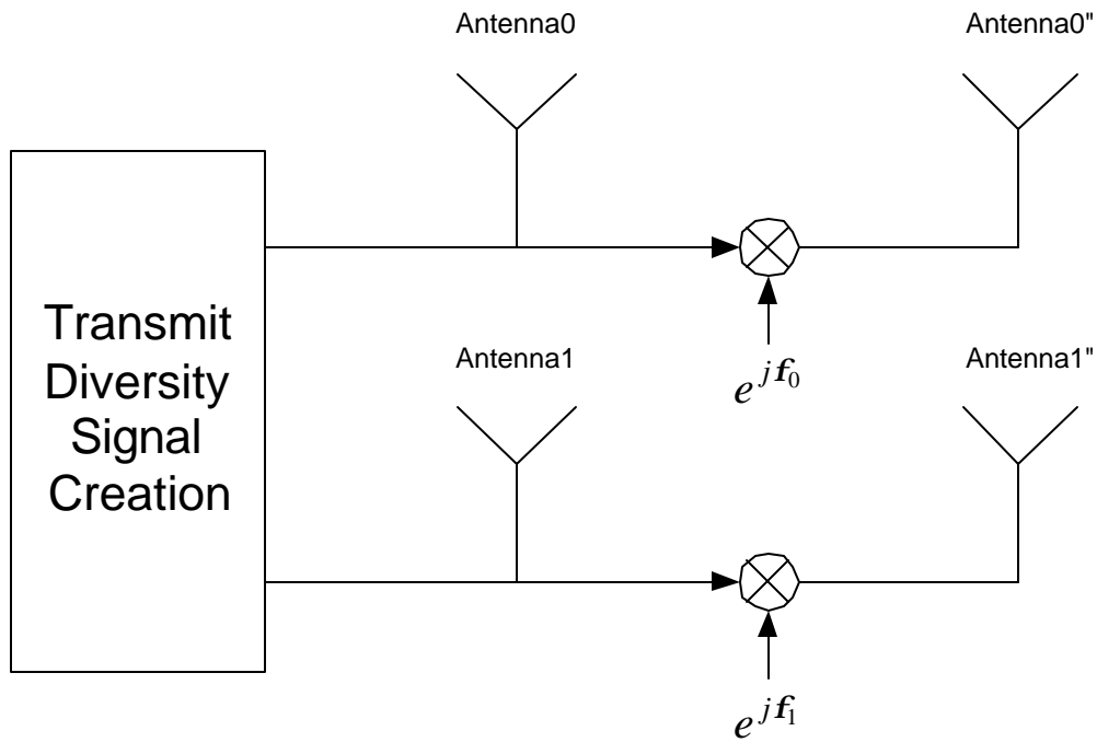
Figure 230b— Illustration of Transmit diversity using 4 antennas
