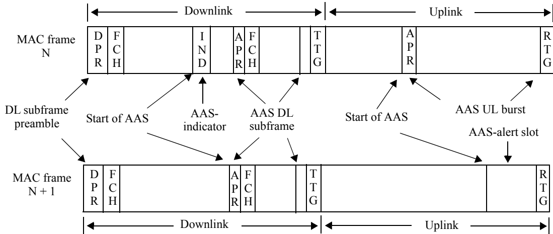
Figure 1—MAC frame contents with AAS elements
