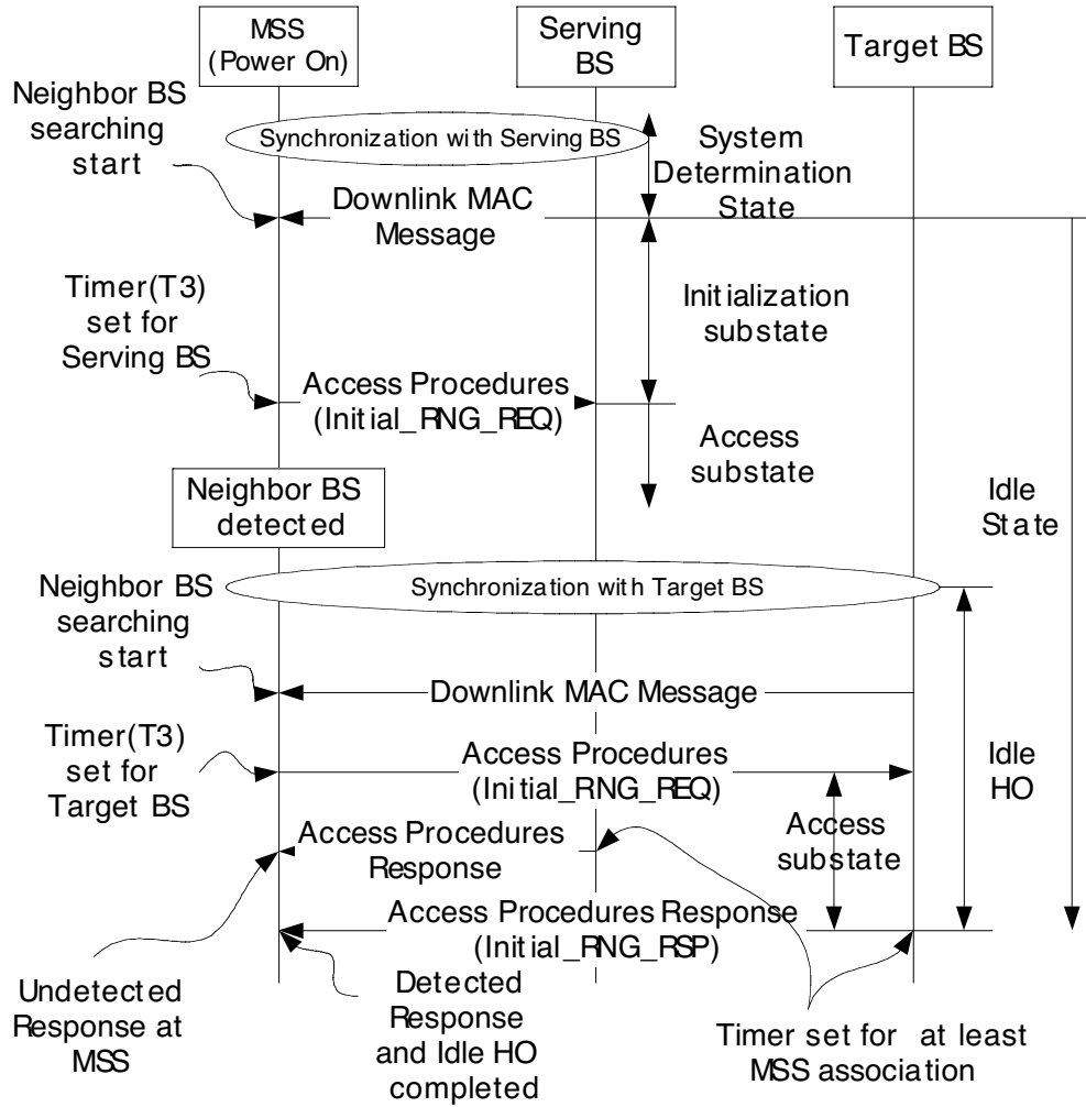
Figure YYY. Call Flow for Idle HO
