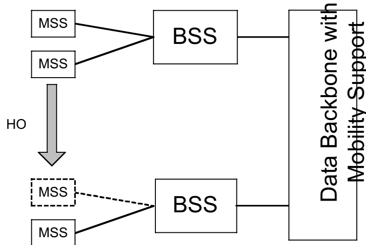
Figure 6: Network Structure (Data Plane) and HO
