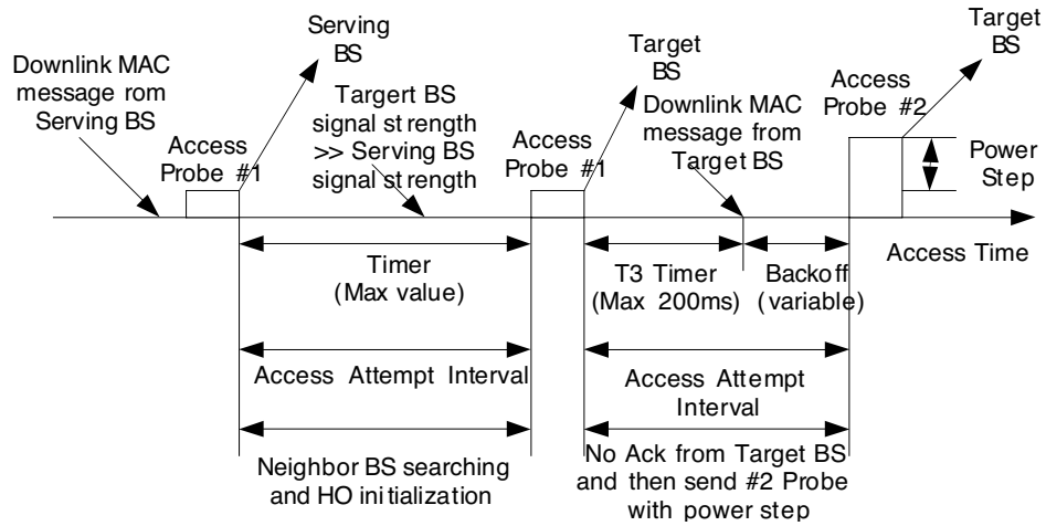
Figure. XXX Idle HO operation
