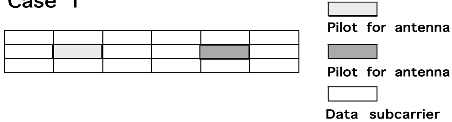
Figure 1 Pilot Allocation Scheme for mini-subchannel type 01 : Case 1
