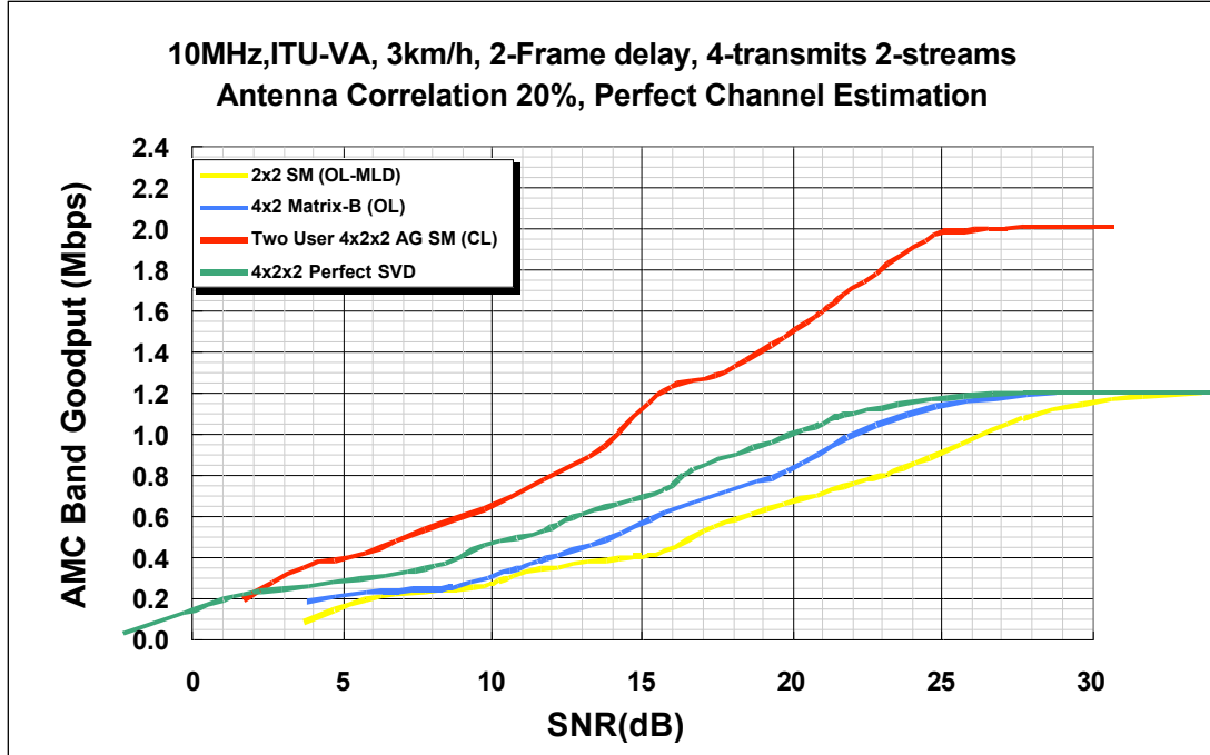
Figure 5 Multi-user Closed Loop AG-SM
