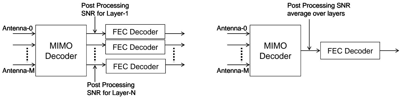
Figure XXX Post processed S/N for MIMO
