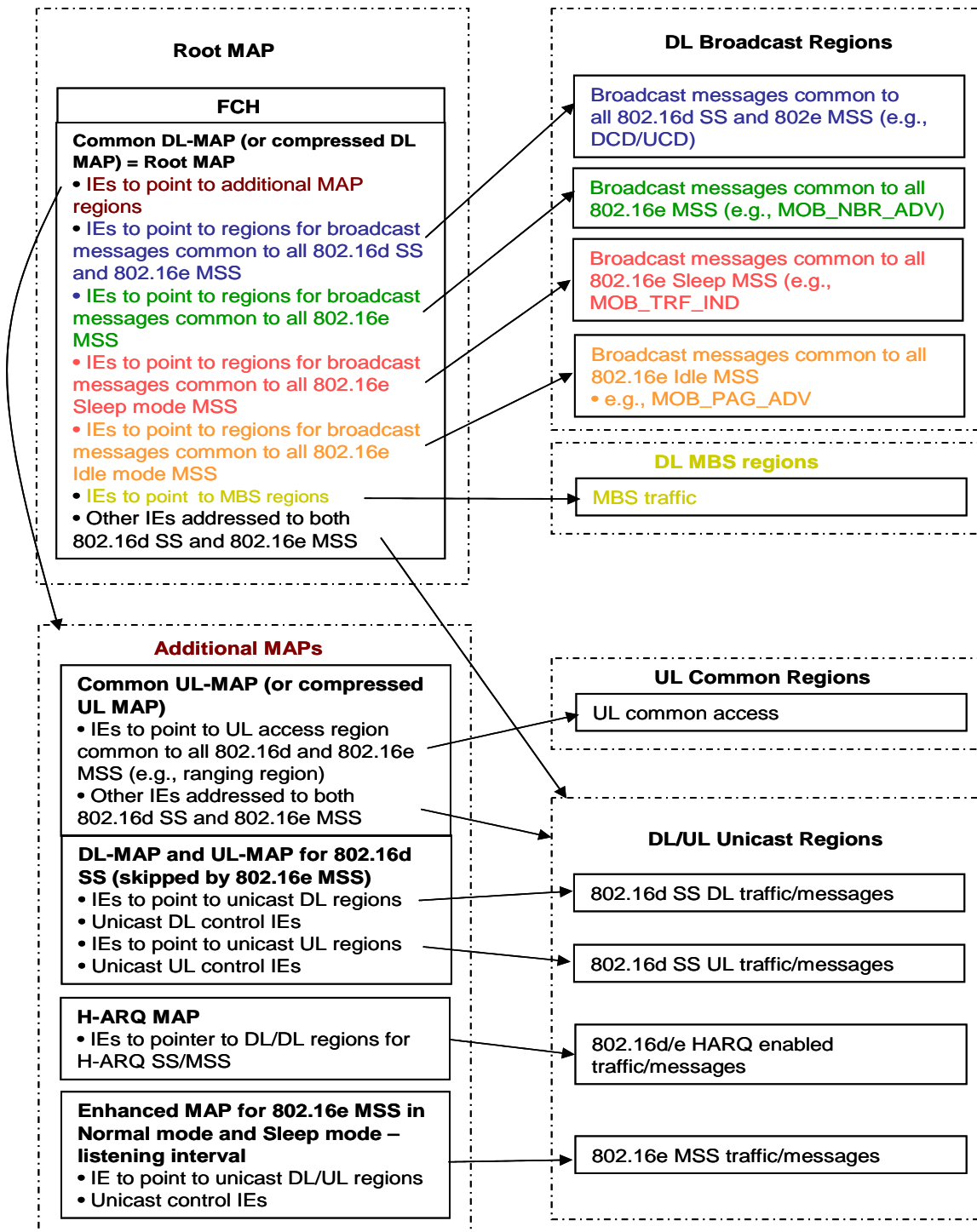
Figure 1. Hierarchical MAP structure
