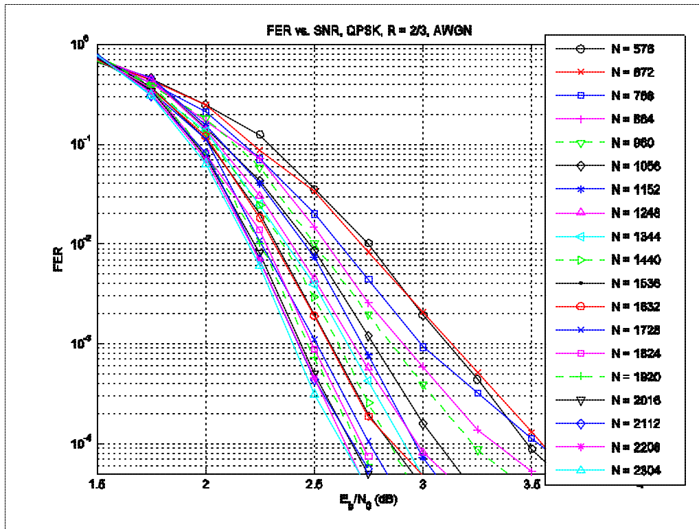
Figure 2. FER vs. E_b/N_0 (dB), QPSK, rate 2/3, AWGN channel.
