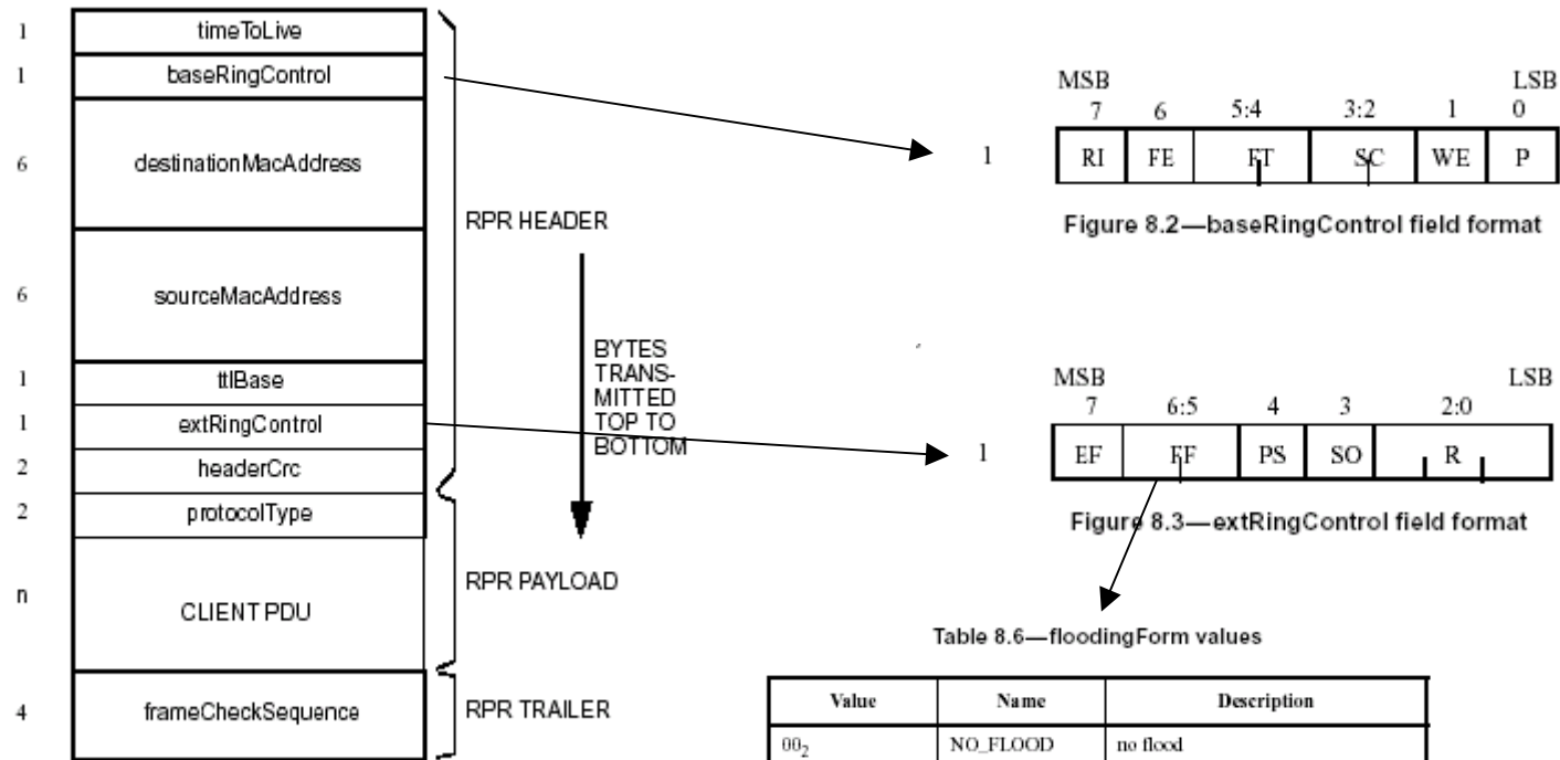
Figure 8.1—RPR data frame format
