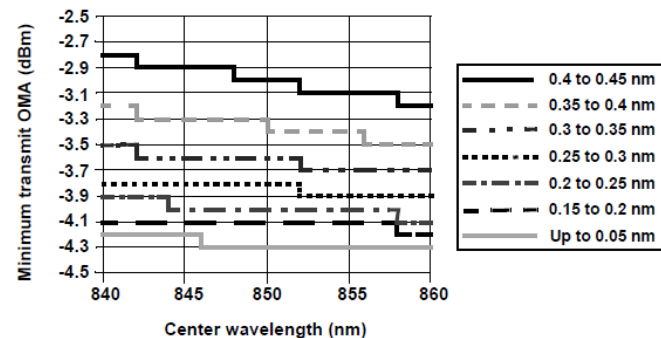
Figure 52-3—Triple tradeoff curve for 10GBASE-S (informative)
