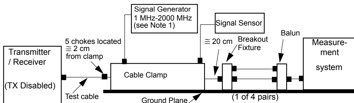
Figure 113A-4—Cable clamp validation test configuration
