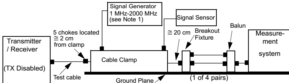
Figure 113A-3—Cable clamp validation test configuration
