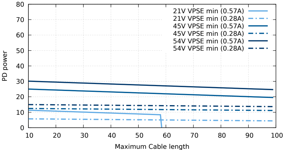
PD power for AWG24, NEC current limited
