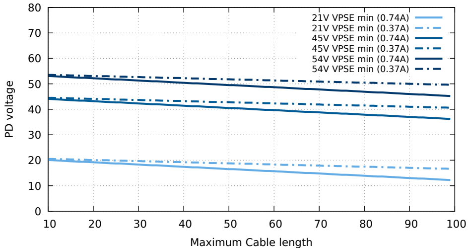
PD input voltage at NEC limits AWG 22
