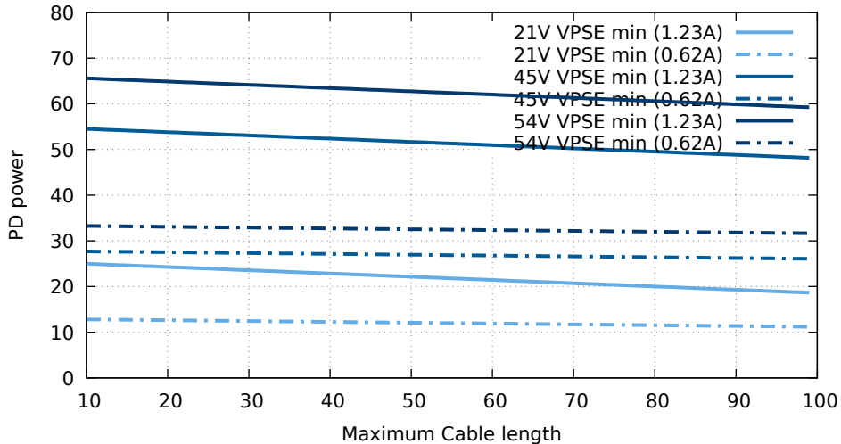
PD power for AWG18, extrapolated current limit
