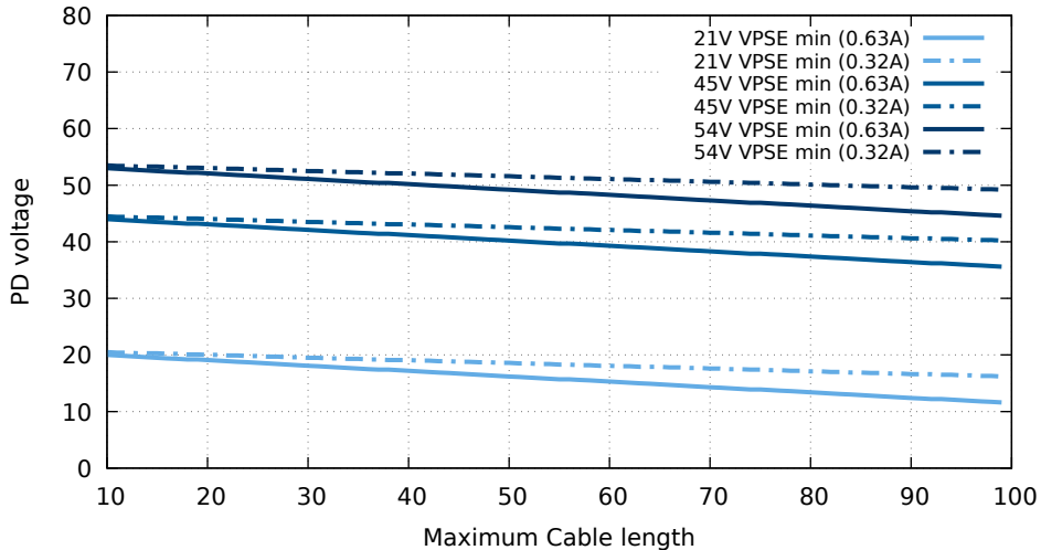
PD input voltage at NEC limits AWG 23
