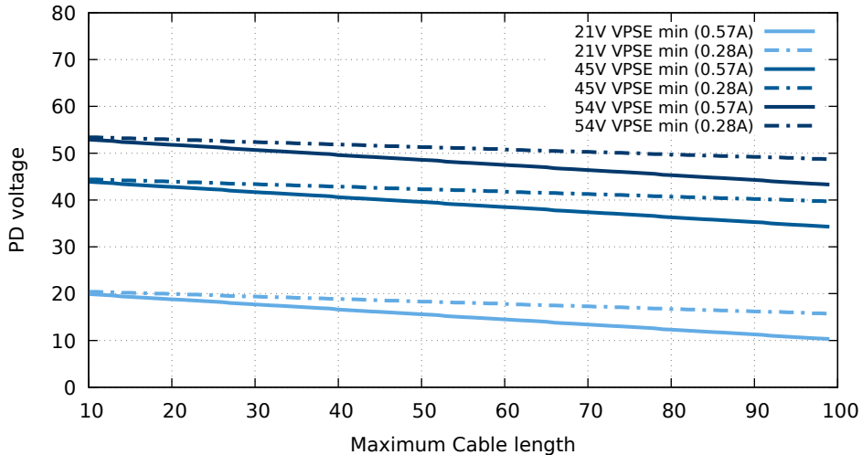
PD input voltage at NEC limits AWG 24
