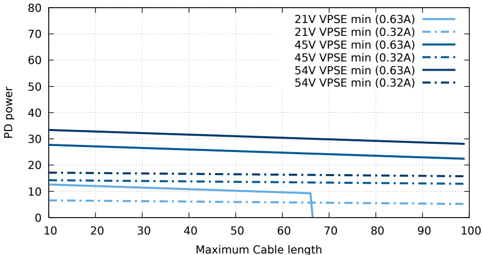
PD power for AWG23, NEC current limited
