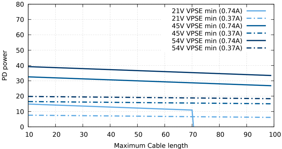
PD power for AWG22, NEC current limited
