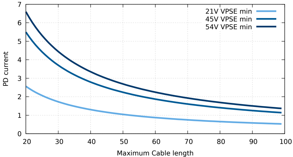
Cable current for AWG22, limited by stability
