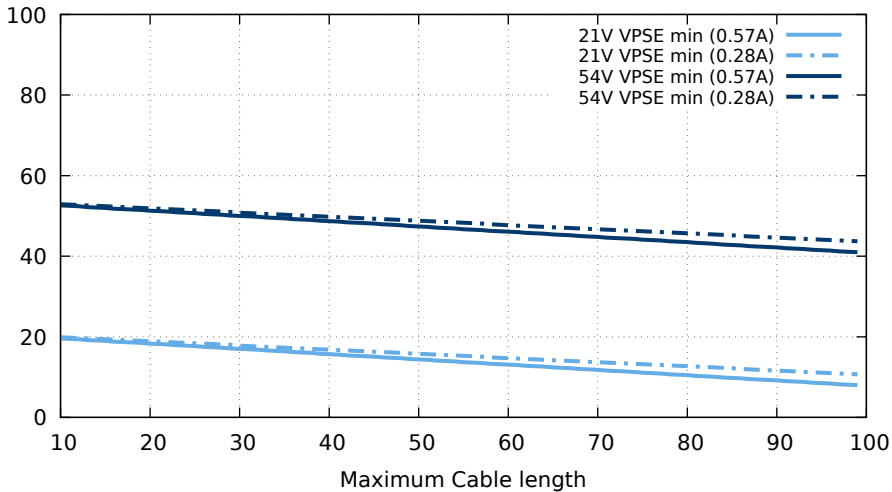
PD input voltage at NEC limits AWG 24
