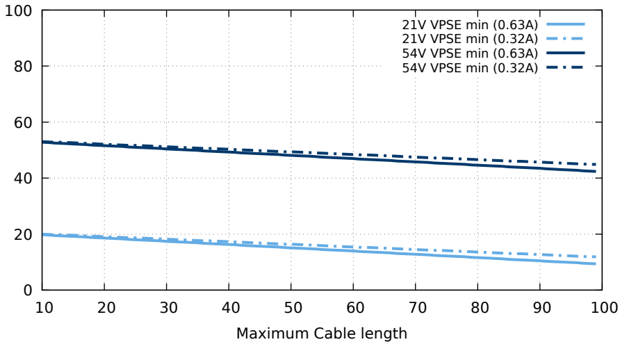
PD input voltage at NEC limits AWG 23
