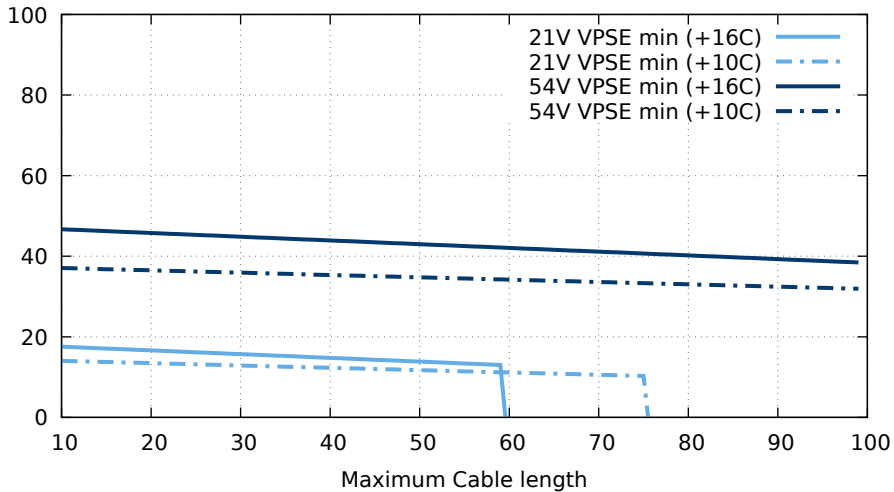
PD power for AWG22, Masood's current limits
