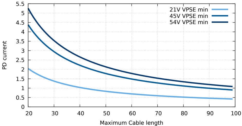
Cable current for AWG23, limited by stability
