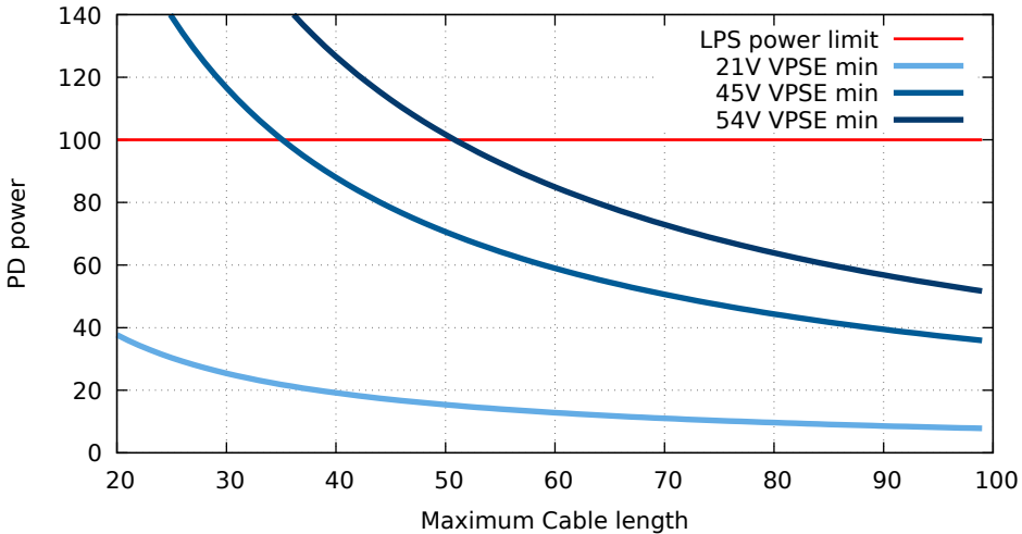
PD power for AWG22, limited by stability
