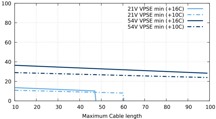
PD power for AWG24, Masood's current limits
