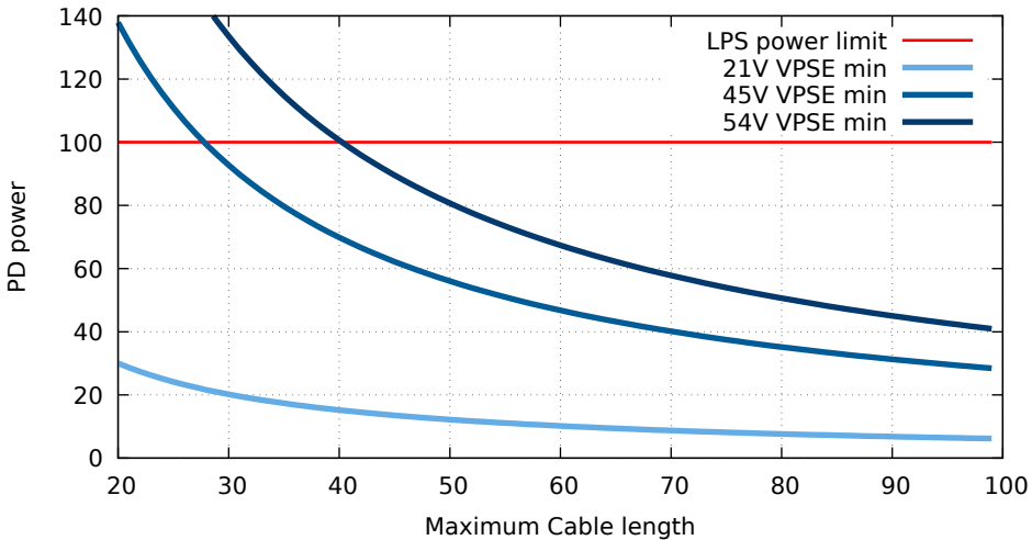
PD power for AWG23, limited by stability
