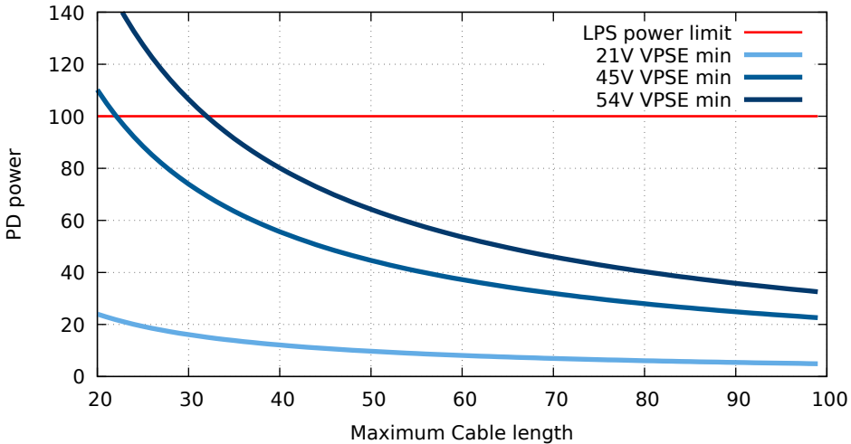
PD power for AWG24, limited by stability
