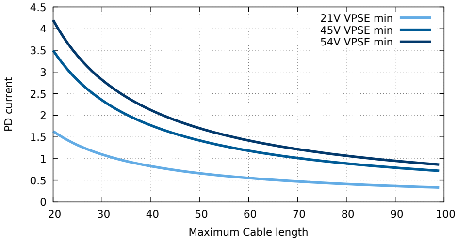
Cable current for AWG24, limited by stability
