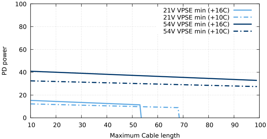
PD power for AWG23, Masood's current limits
