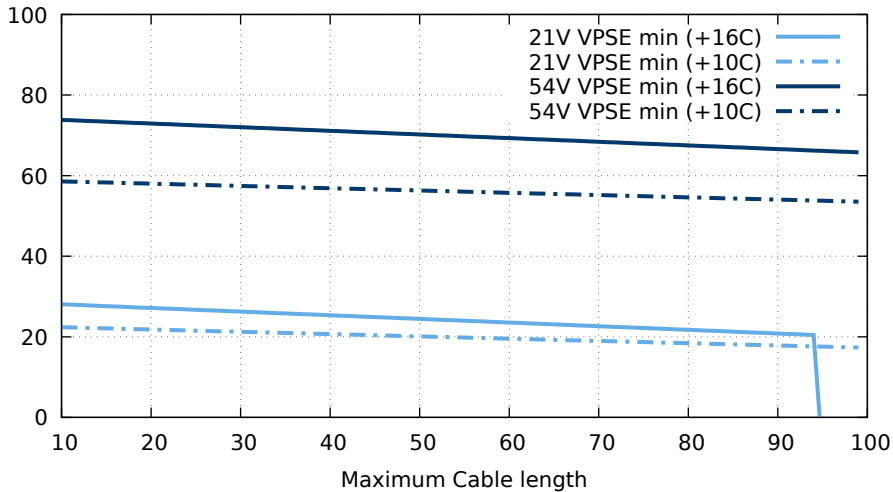
PD power for AWG18, extrapolated current limit
