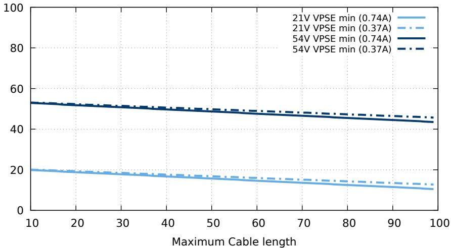
PD input voltage at NEC limits AWG 22
