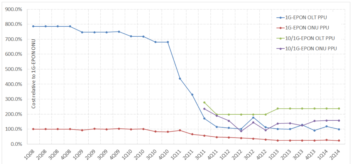
Figure 1: Relative cost of 1G-EPON and 10/1G-EPON ONU and OLT devices over time
