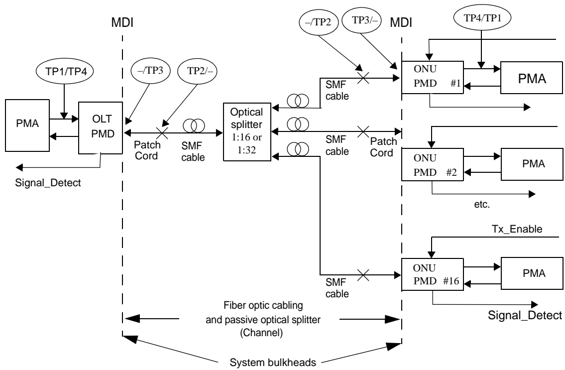
Figure 91-3—10GBASE-PR and 10/1GBASE-PRX block diagram
