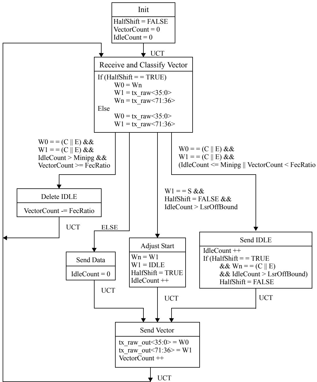
Figure 92–8—ONU Alignment / Idle Detector state diagram
