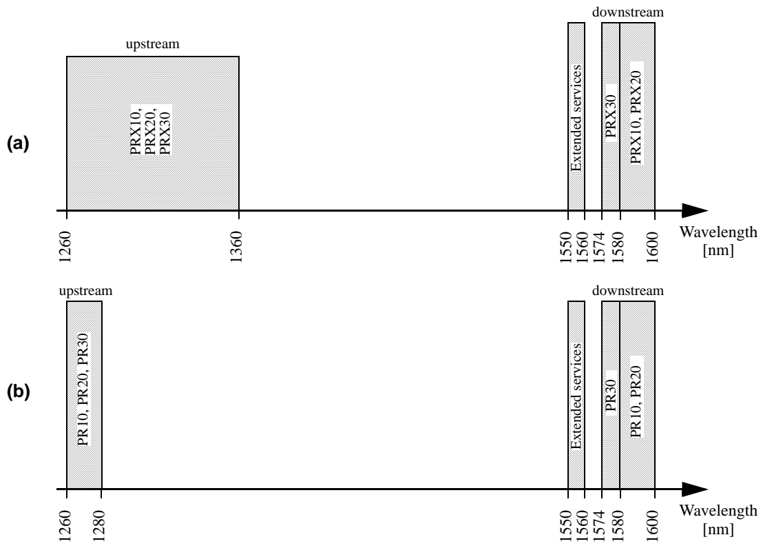
Figure 75-8—Wavelength allocation plan for (a) PR and (b) PRX type PMDs.
