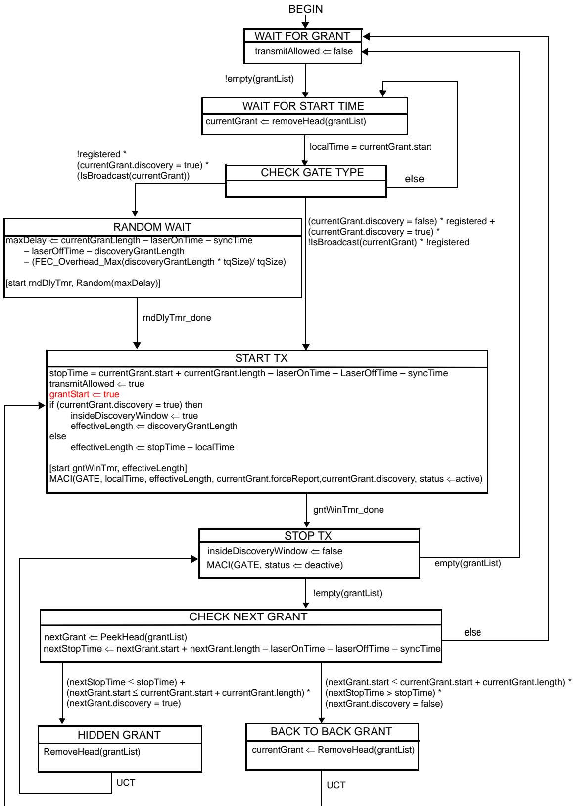
Figure 77–29—Gate Processing ONU Activation state diagram
