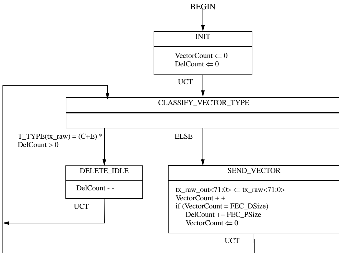
Figure 76-9—OLT Idle Deletion state diagram
