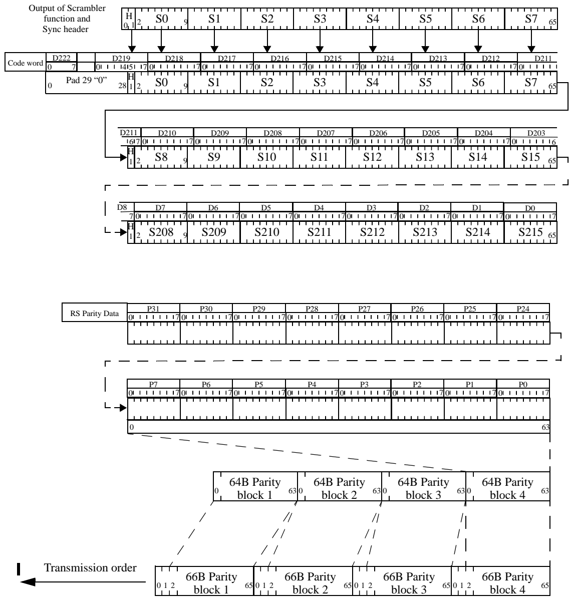
Figure 76–12—Bit ordering in FEC codeword generation
