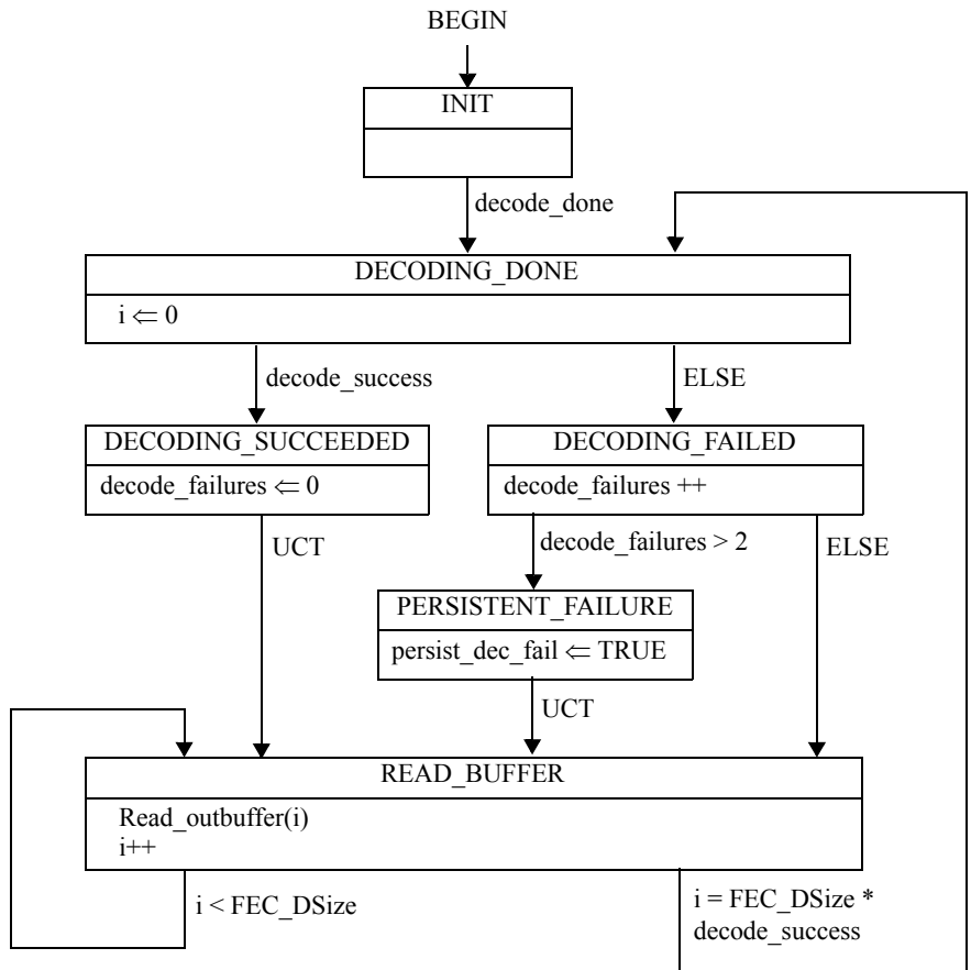
Figure 76-21—FEC codeword processing state diagram
