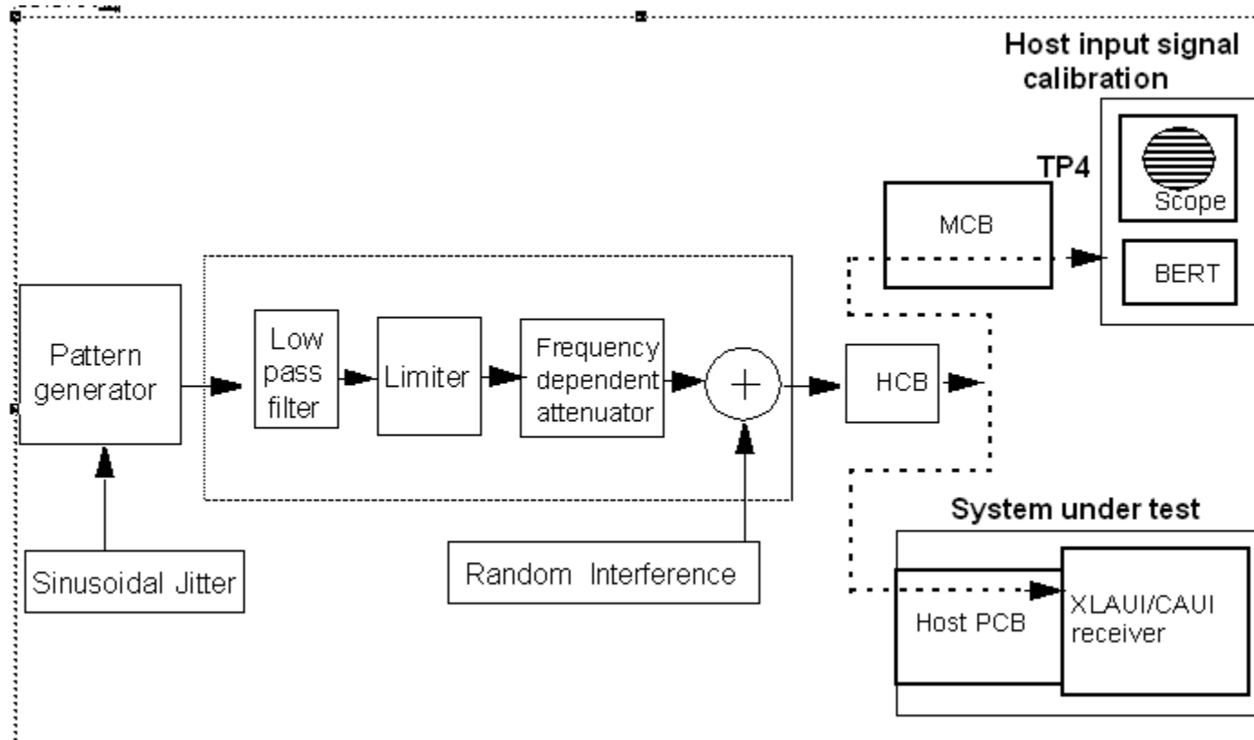
Figure 83B-10 Stressed-eye and jitter tolerance test setup
