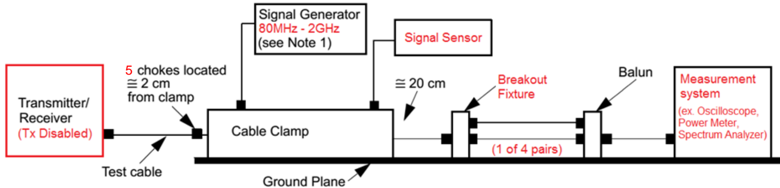
Figure 113A-3 - Cable clamp validation test configuration
