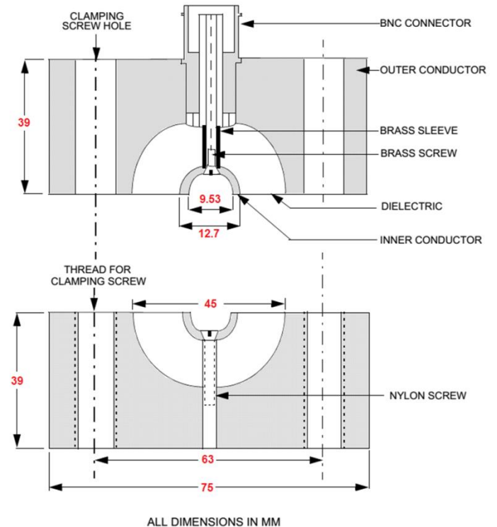
Figure 113A-2 - Cross-section of cable clamp
