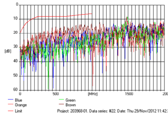
RETURNLOSS-Channel#1-Fromequipmentend.f
