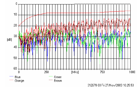
4.3 High frequency transmission test results. Channel #3 (15m hrzt), from terminal end RETURN LOSS Data series #12
