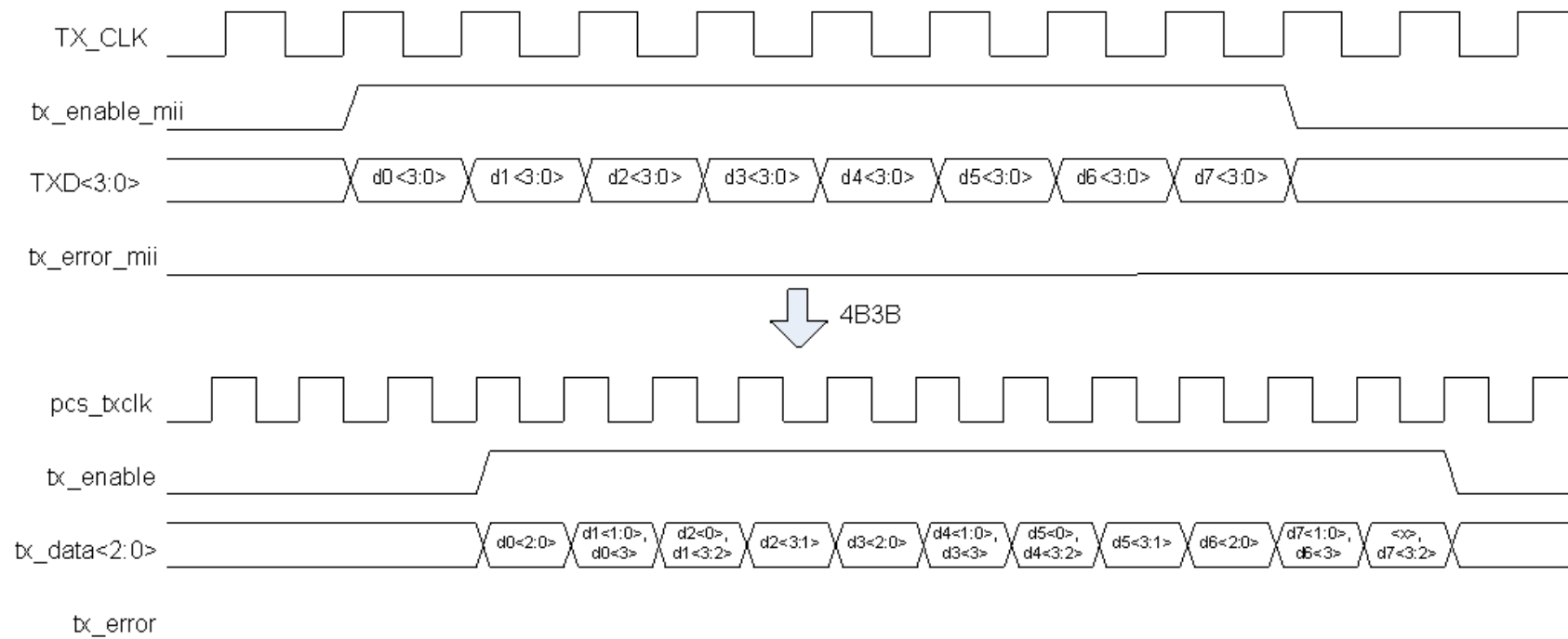
Case 3: 4B3B MII signals conversion ( (3n+2)-bit data, one stuff bit appended)
