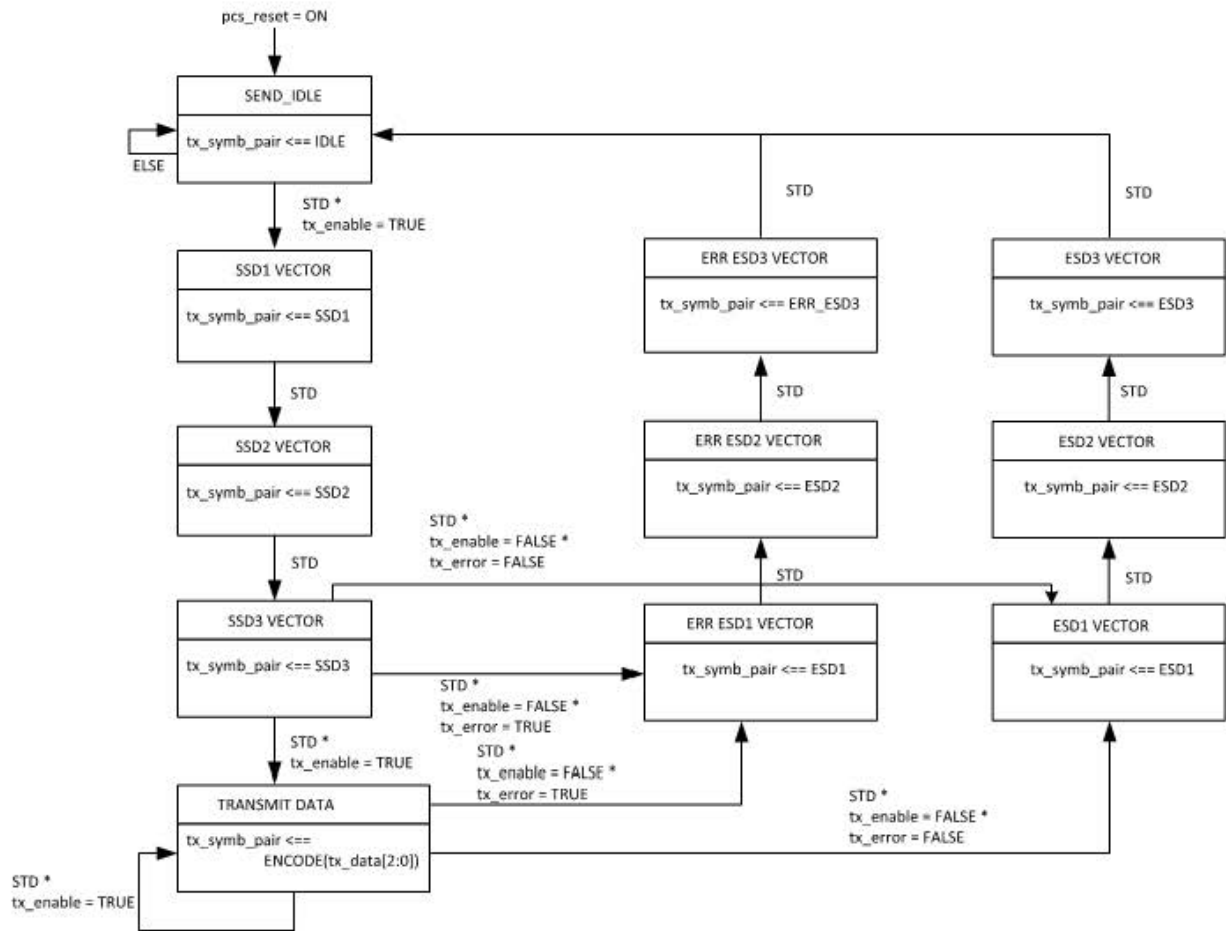
Figure 96-6---- PCS Transmit State Diagram
