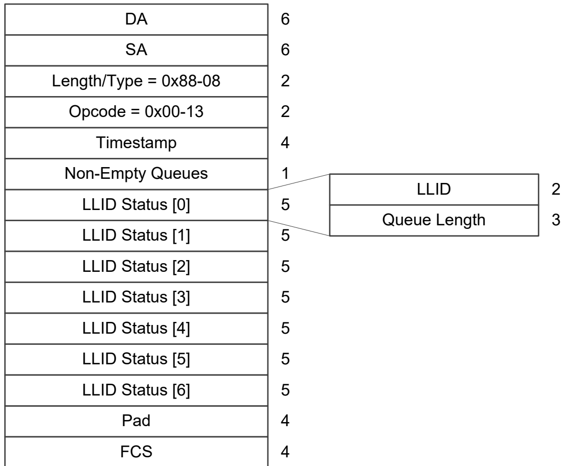
Figure 144-21 – REPORT MPCPDU
