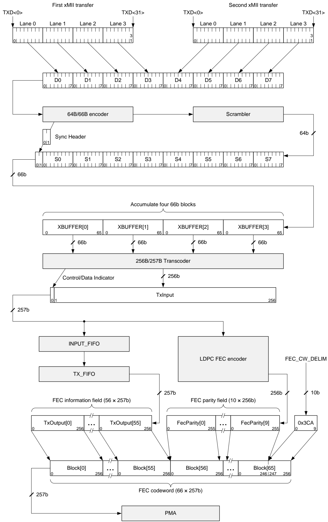
Figure 142-5 – Transmit bit ordering
