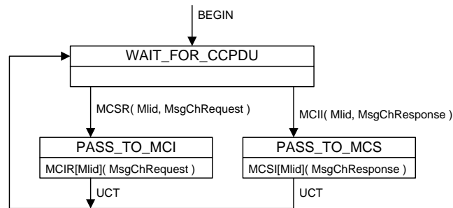
Figure 144-29 – OLT CCPDU Processing state diagram
