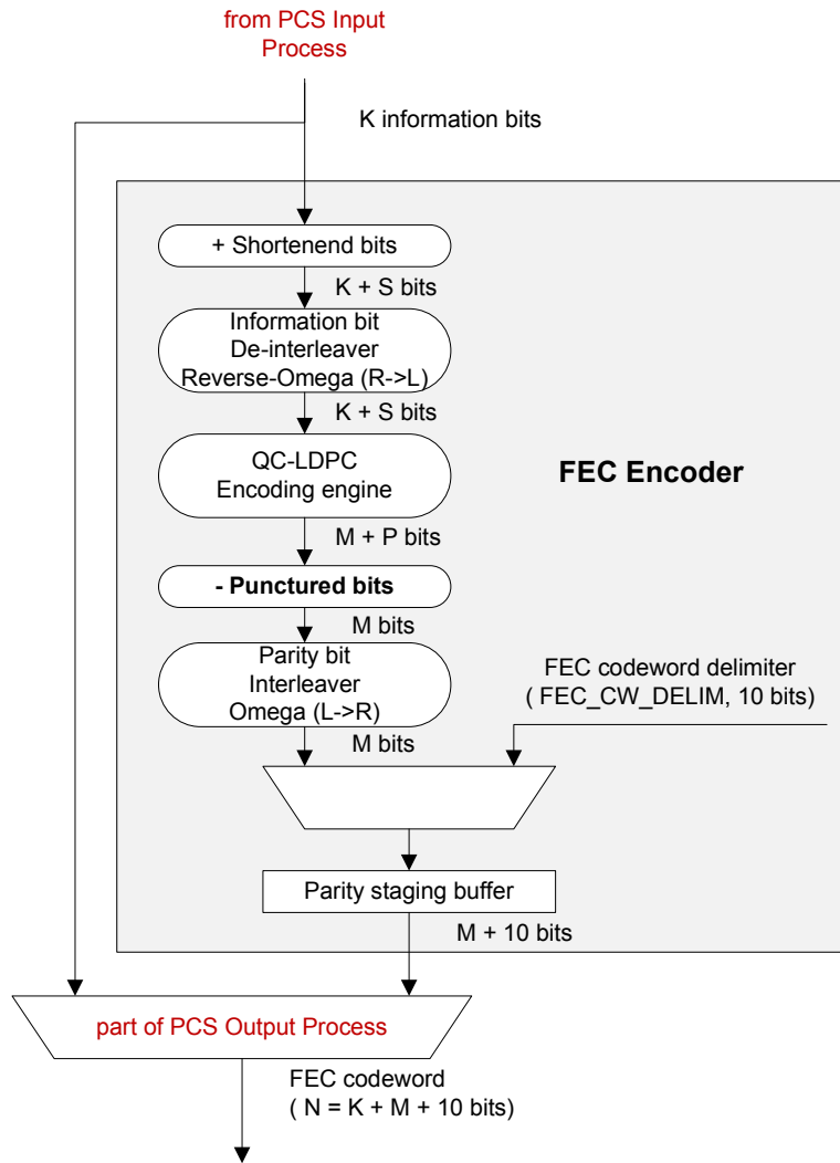
Figure 142-6—FEC encoder
