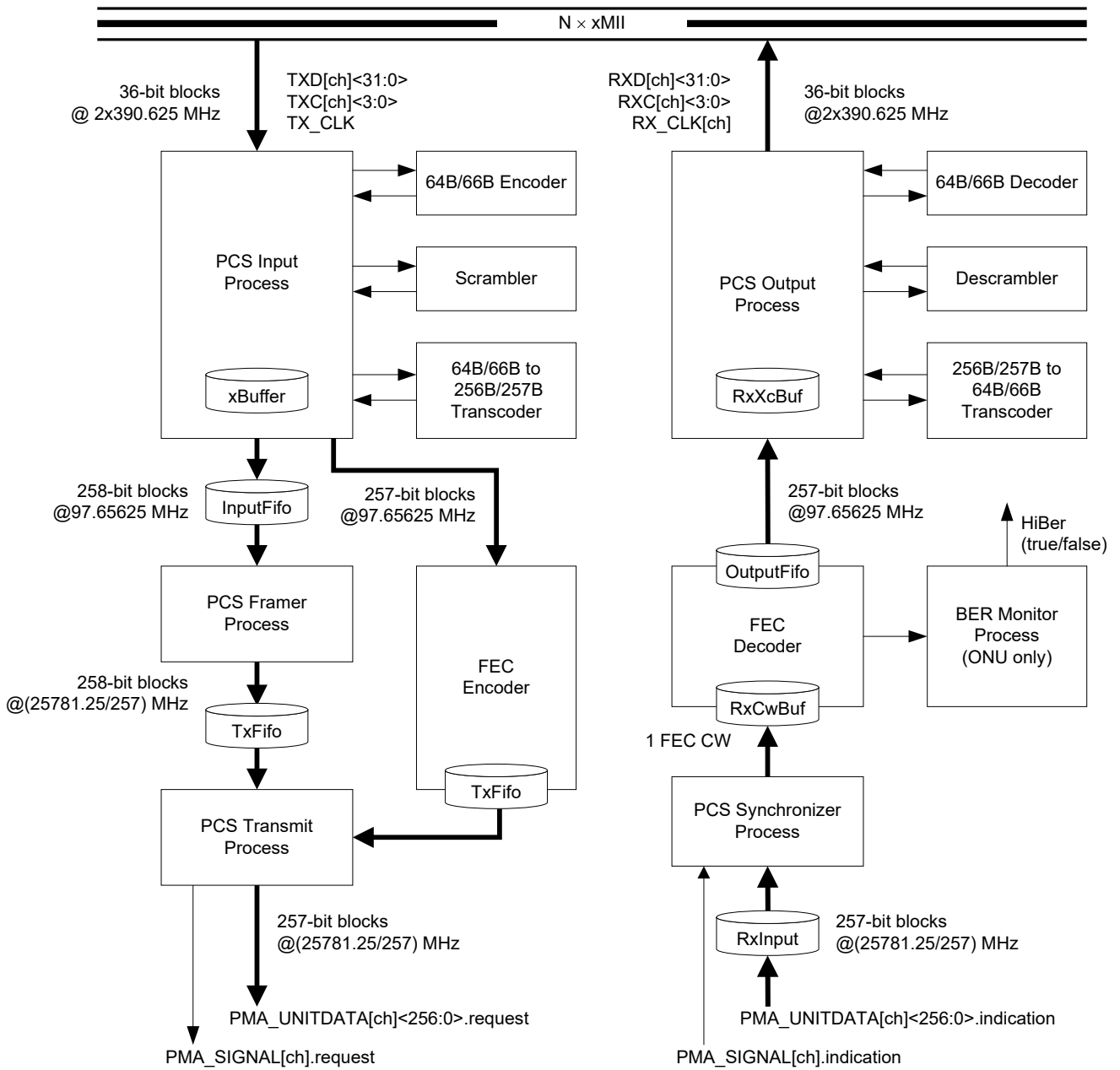
a) PCS transmit path
