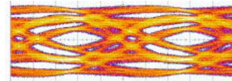
Uncompensated F2: 300m, BER varying between 1e-5 to 1e-9 (Offset launch)
