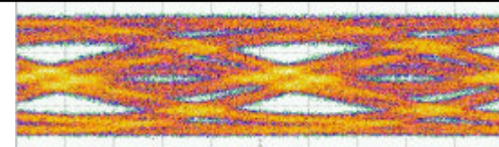
Uncompensated F1: 400m, Error Floor at 1e-3 (Center launch)
