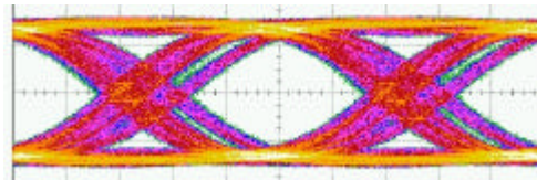
Compensated F2: 300m, BER < 1e-12 for Tx power > -3.5dBm (Offset launch)
