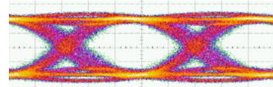
Compensated F1: 400m, BER < 1e-12 for Tx power > -3dBm (Center launch)
