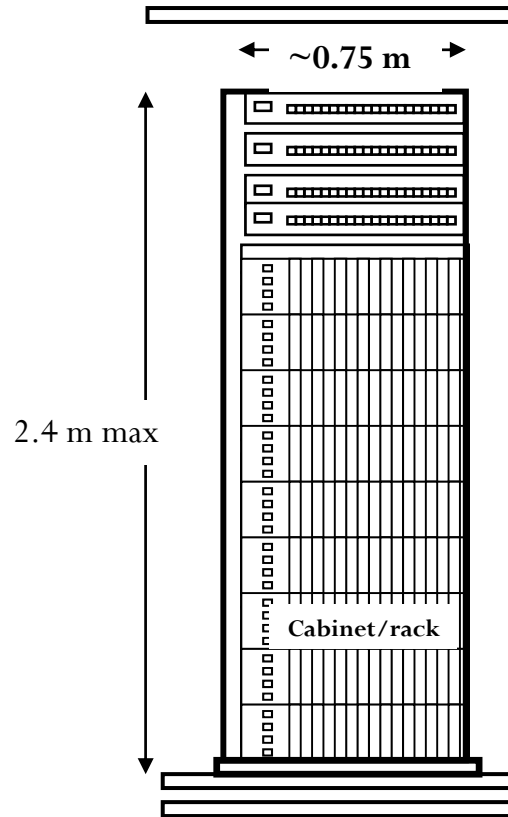
Intra-rack configurations
