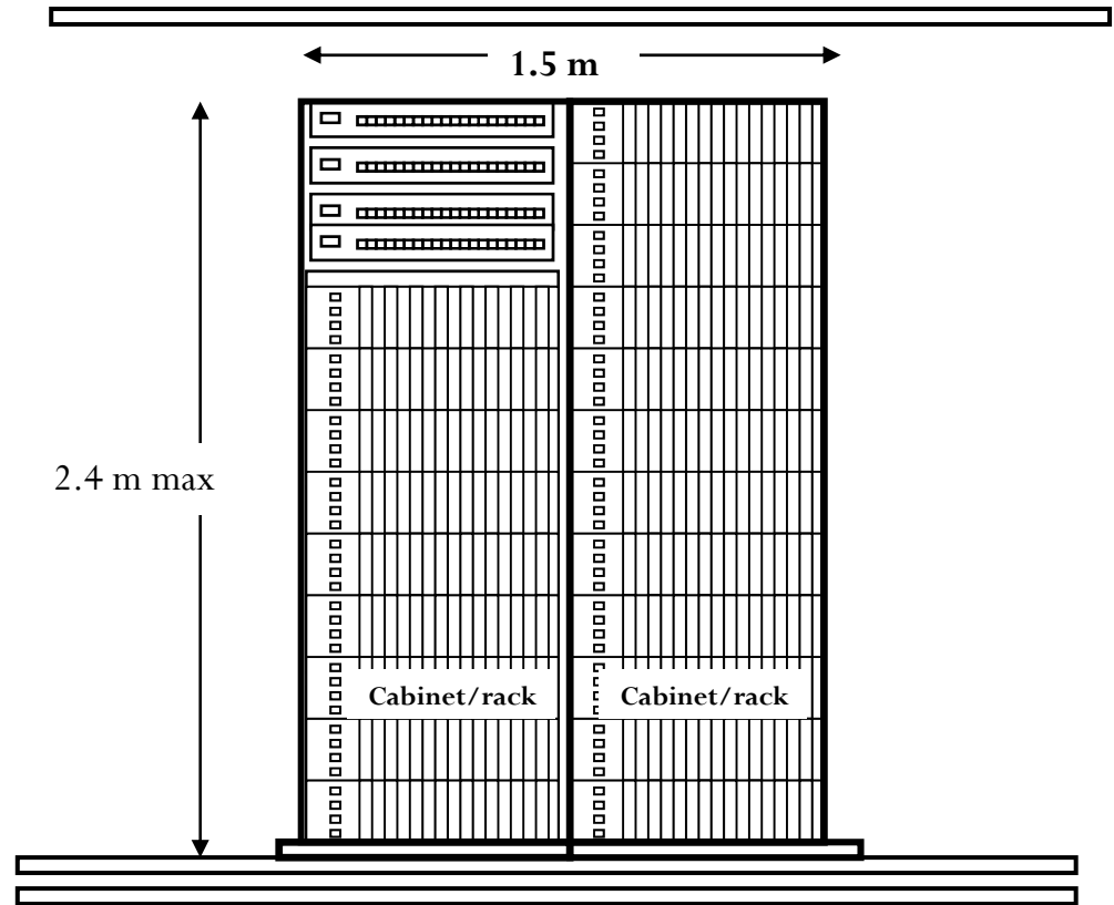
Inter-rack configurations
