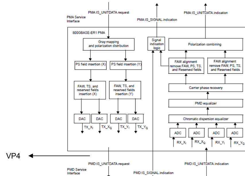
Figure 186A-2 Test vector points for 800GBASE-ER1 PMA
