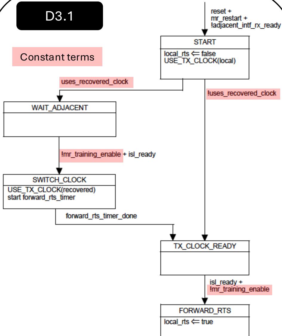
Figure 178B-9—RTS update state diagram
