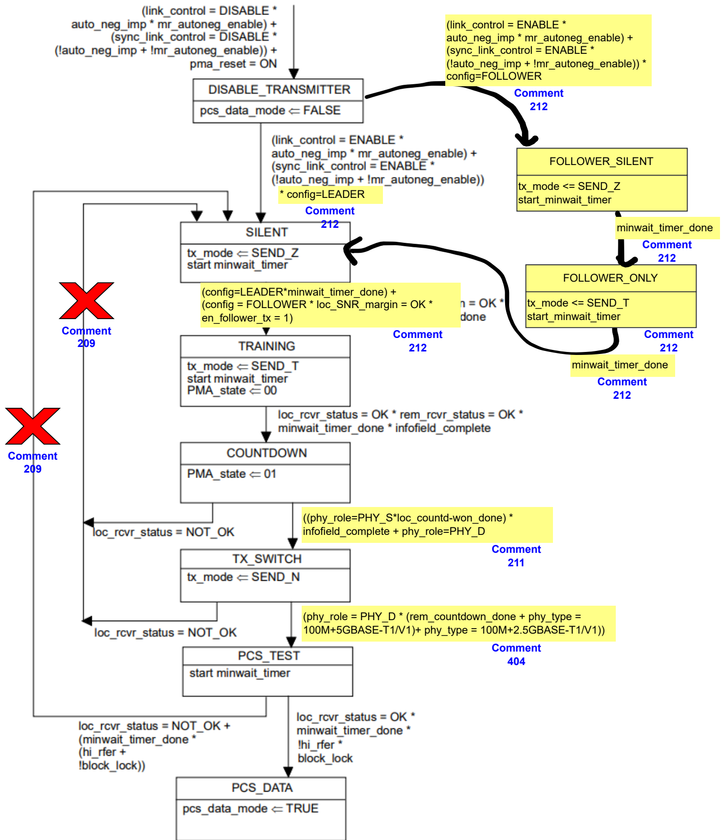
Figure 201-17—PHY Control state diagram
