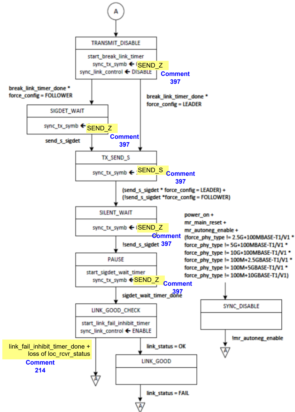
Figure 201–20—PHY Link Synchronization state diagram
